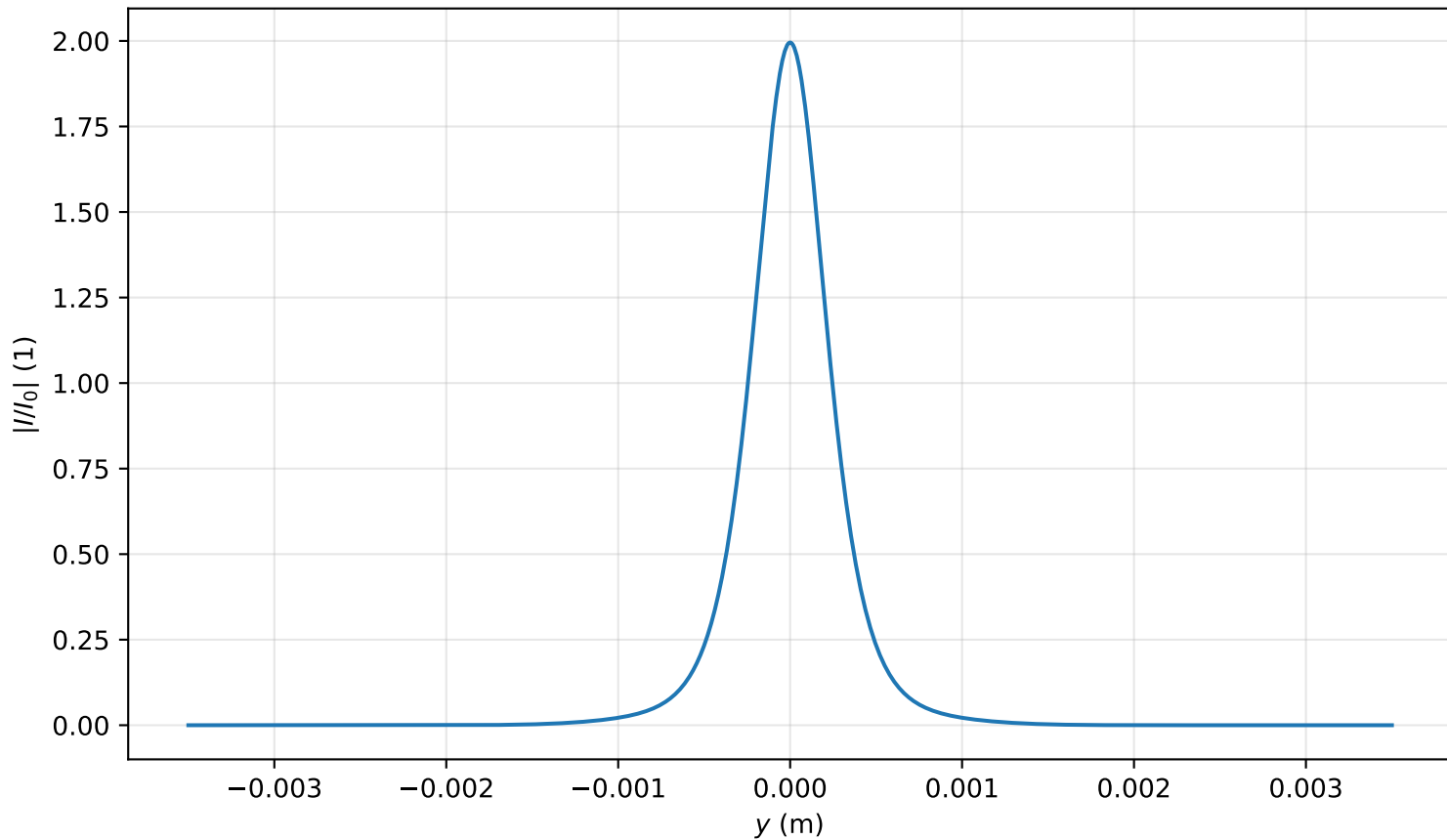
Intensity profile I(x=0, y, z=1.751)/I_0 , P_{in}=1.0P_{cr} , artificial time
